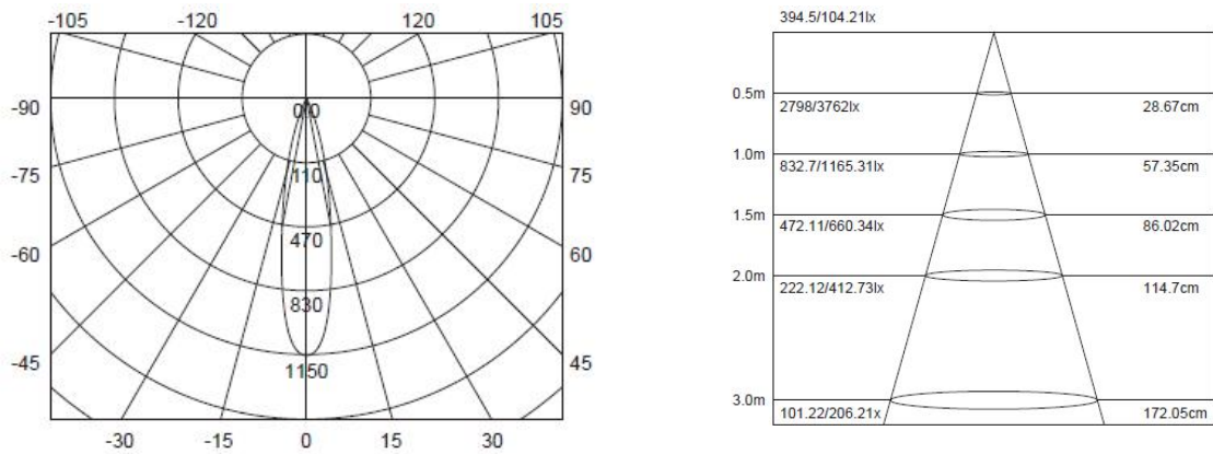
Beam Angle 24° cd&lx
