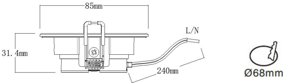
Technical Drawings (L/N wire 240mm)
