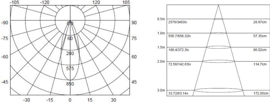
Beam Angle 36° cd&lx
